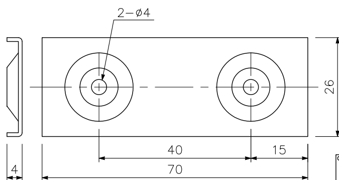
Joint Bracket
