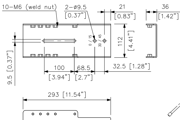
Mounting base
