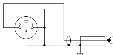
Plug Diagram
