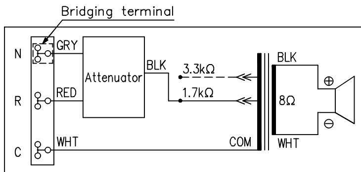
3-wire connection
