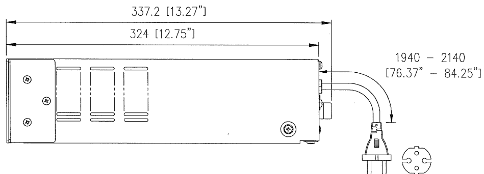
Right View
