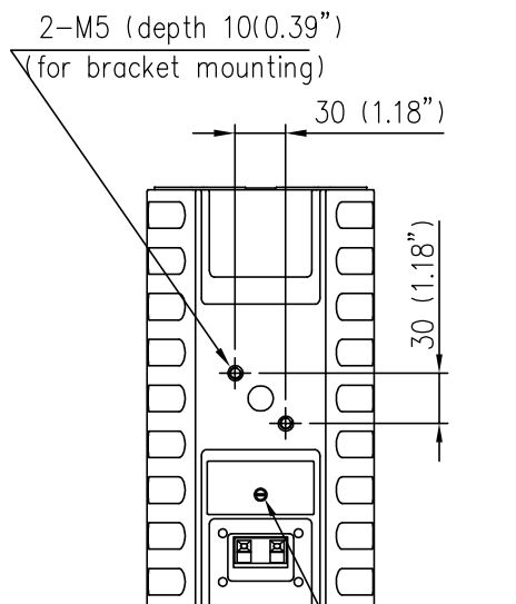
Rear View
